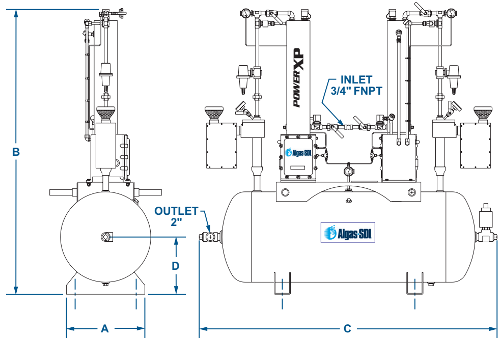
File:XPVSPEC1.DWG
